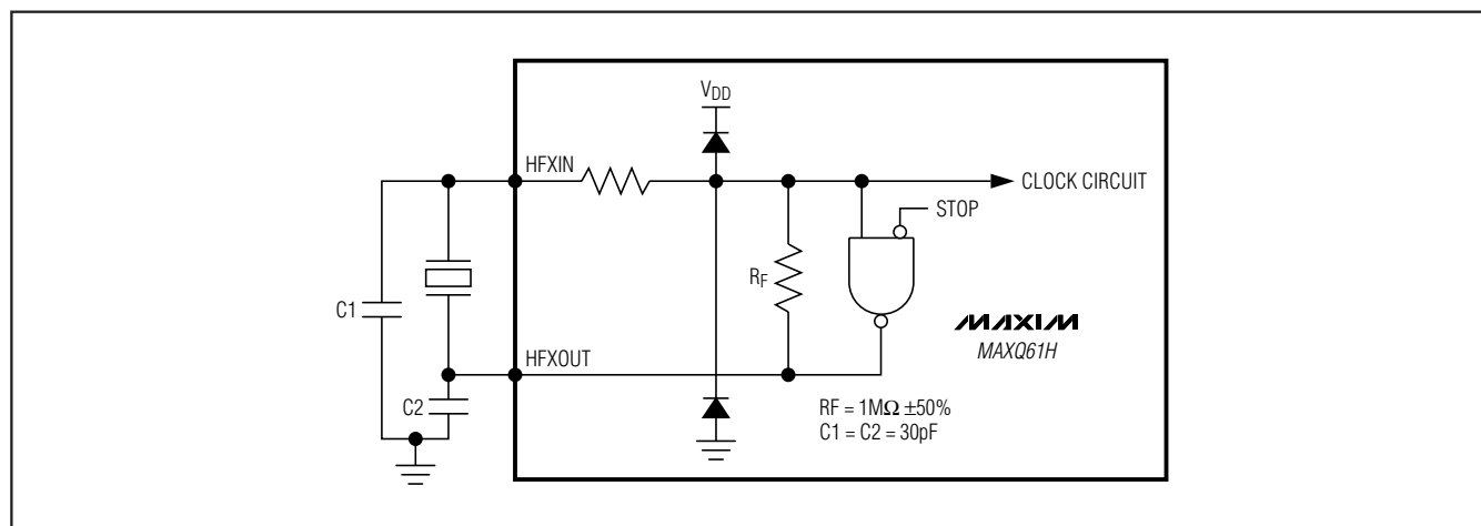
Figure 7. On-Chip Oscillator
